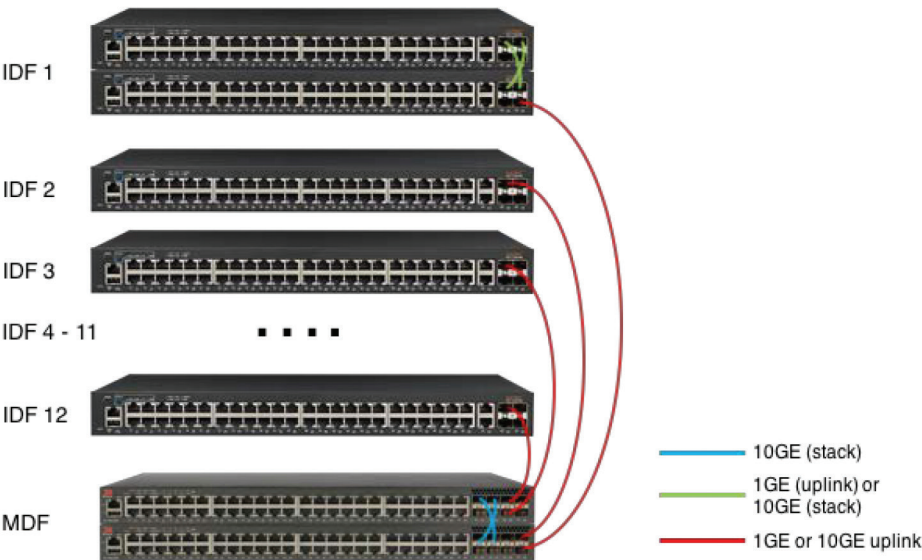
Figure 3. Typical 12-IDF design with dual-core MD
